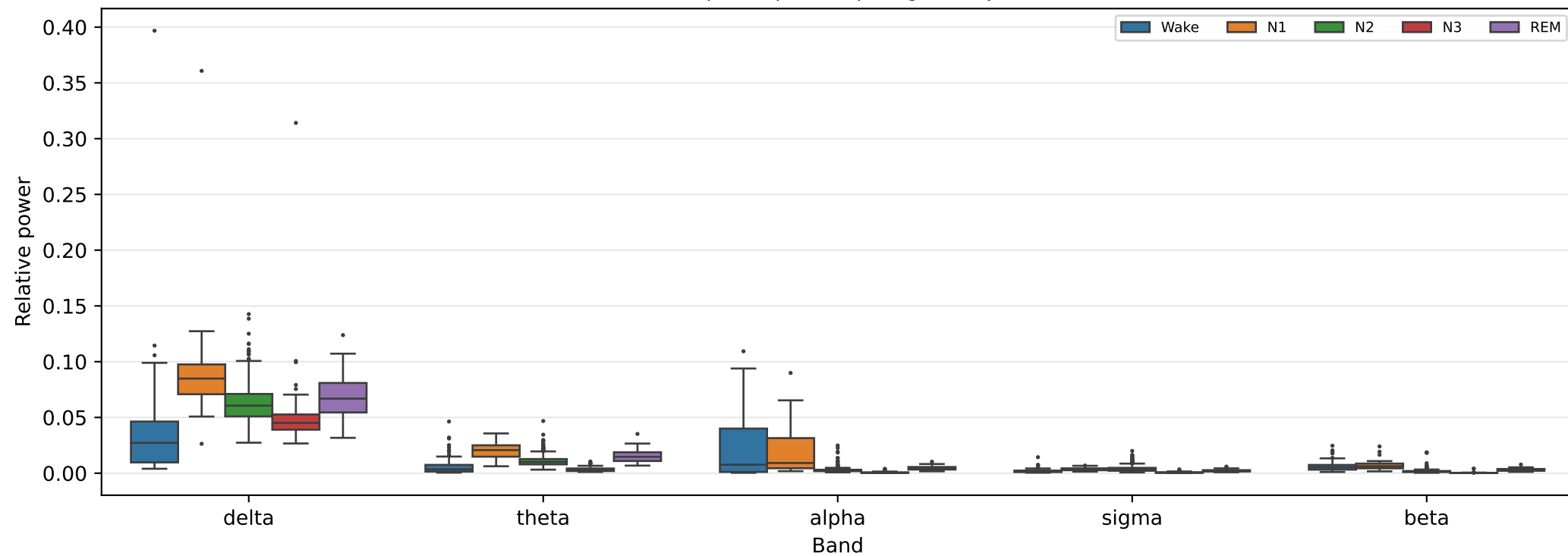
Relative band power per sleep stage - subject 6, Pz-Oz
